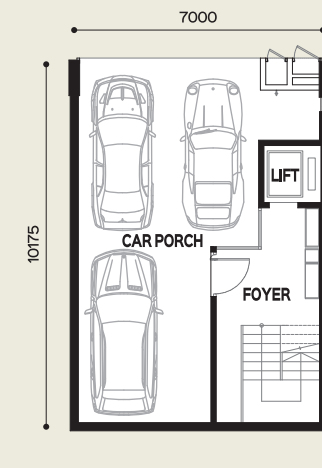
LOWER GROUND FLOOR PLAN
